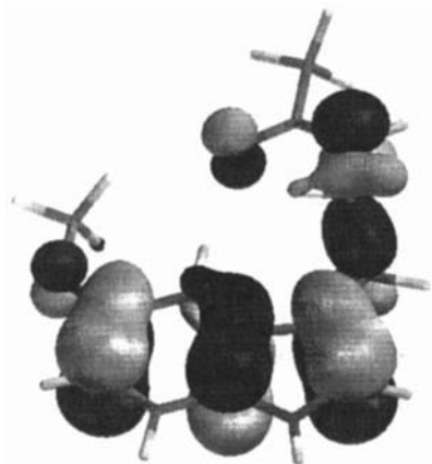
Fig. 3. SOMO of the melatonin radical cation ( 1Bu •+ ) according to AM1 calculations
